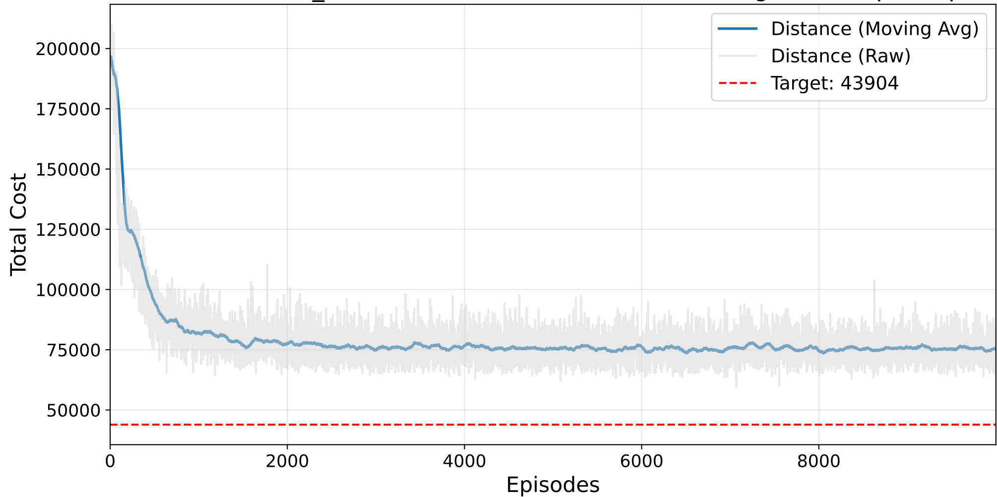
Final RANDOM_SEARCH Masked AutoRL-SOP Training - kro124p.3.sop
